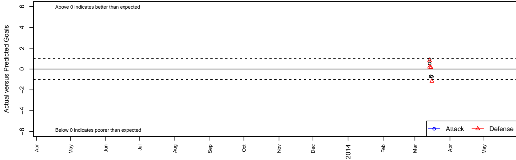
Hawaii Rush 99 Nero B98 Dots are actual minus expected GF (blue circles) and GA (red triangles). Blue line is smoothed change in attack strength. Red is smoothed change in defense strength.
